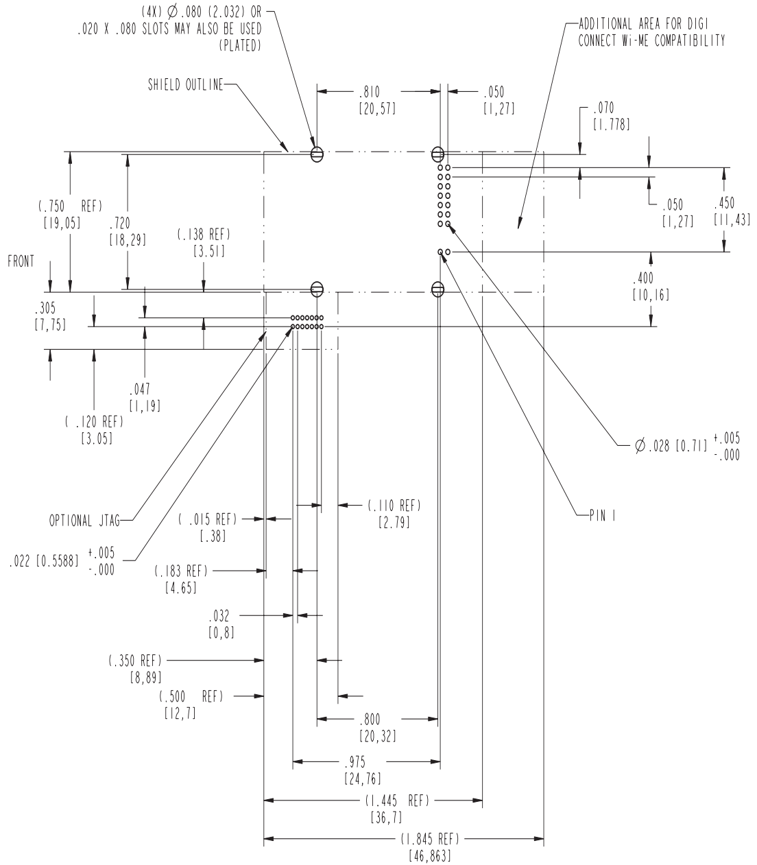
RECOMMENDED PCB LAYOUT TOL. \pm .005 [0,127] NON-CUMULATIVE
